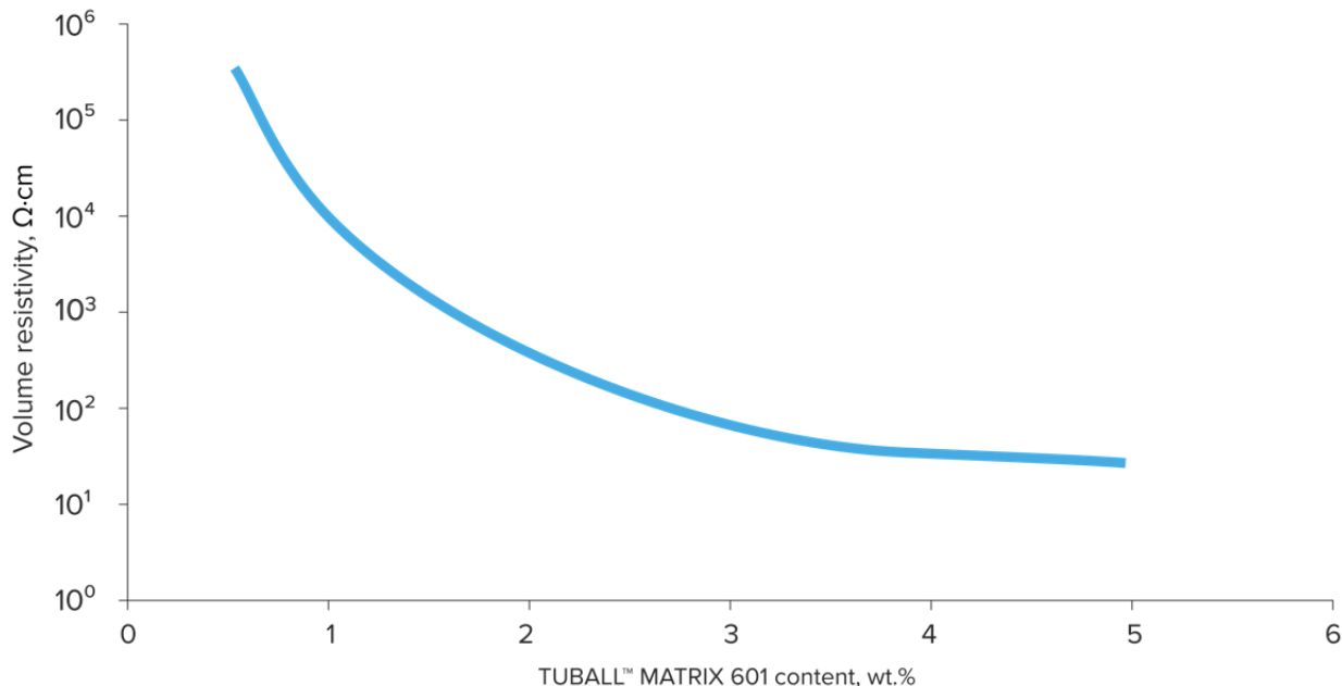
Figure 1. Volume resistivity of RTV with TUBALL™ MATRIX 601 is in the range 10 1 –10 5 Ω·cm*
